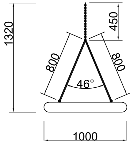
① SIDE VIEW
