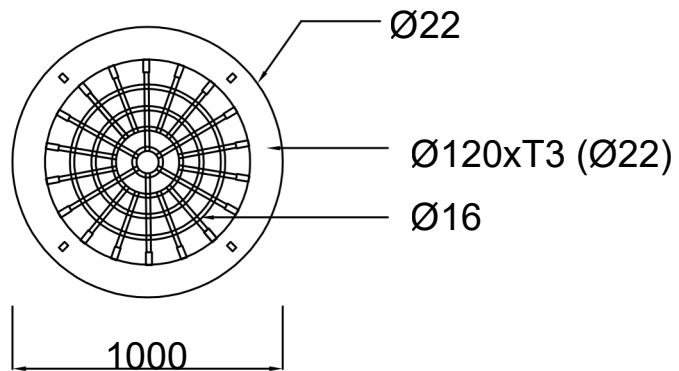
③ TOP VIEW
