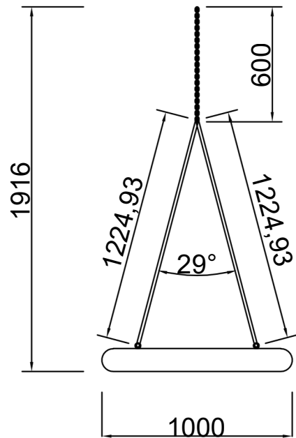
① SIDE VIEW
